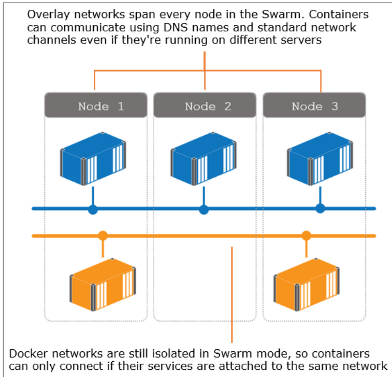
Figure 12.12 Networks in the Swarm span the whole cluster and still provide isolation between apps
