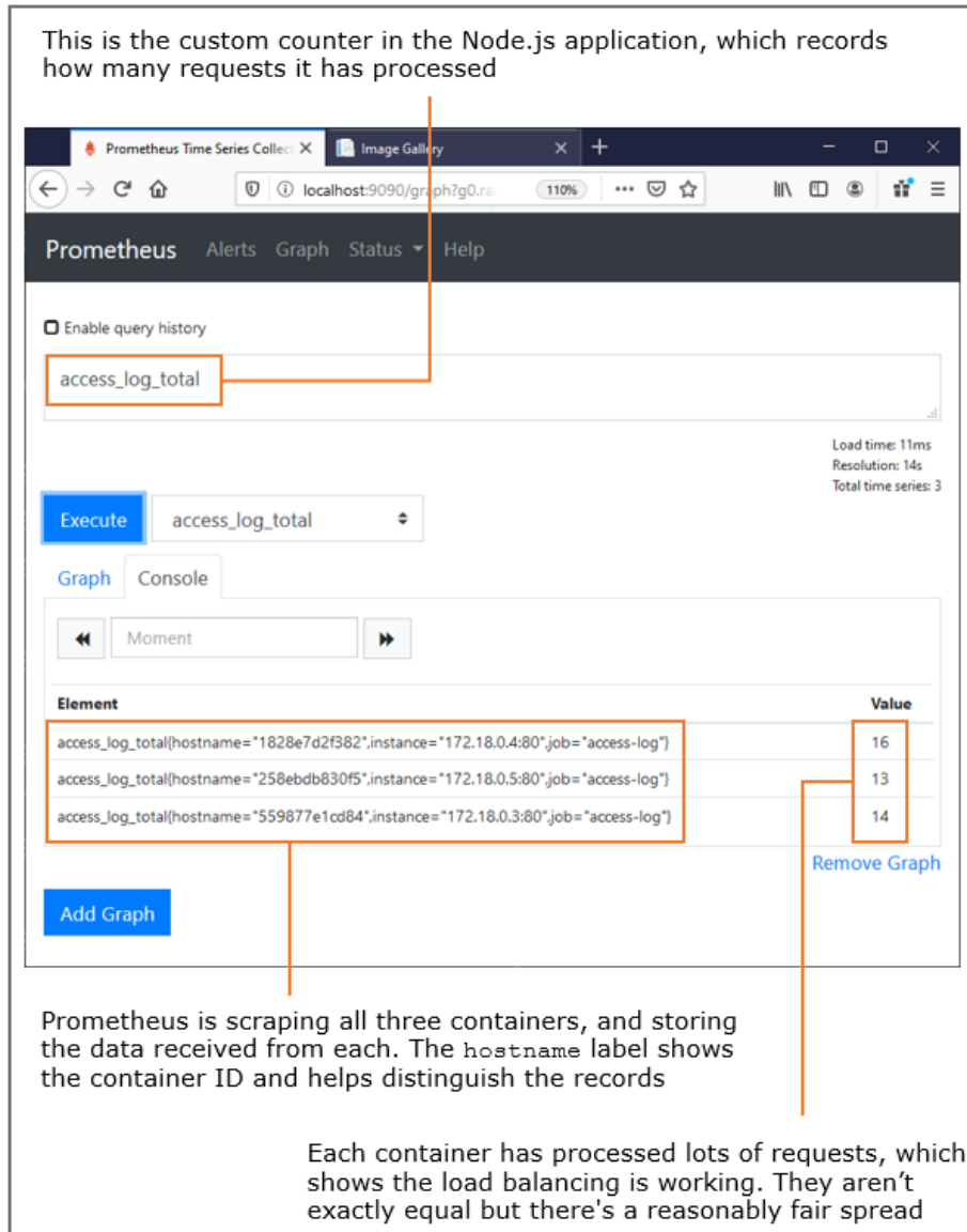
Figure 9.9 Processing metrics can be used to verify that requests are being load balanced
