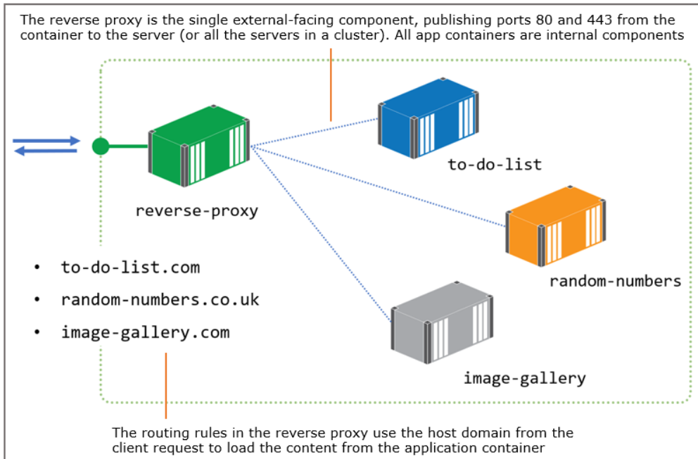
Figure 20.16 Using a reverse proxy to host many applications with different domain names in one cluster
