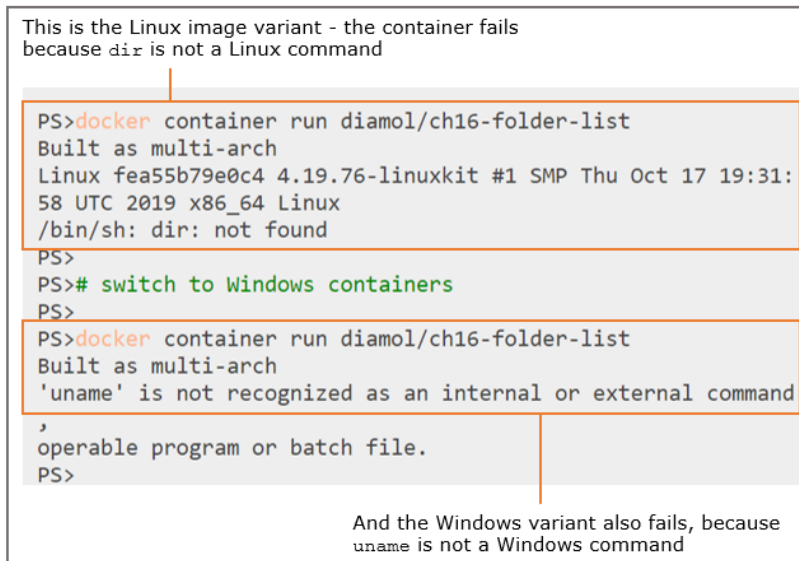
Figure 16.7 It's easy to build a multi-arch image which fails at runtime on some platforms
