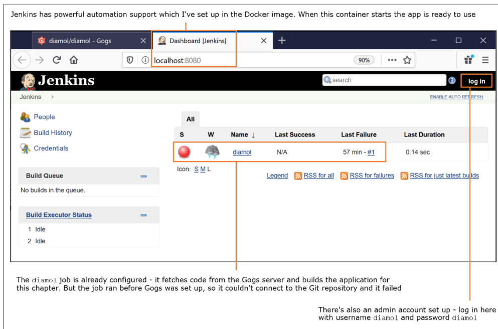
Figure 11.6 Running Jenkins in a container - it is fully configured with a user and CI job already set up
