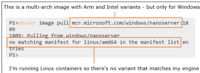
Figure 16.3 You can't pull an image from a registry if there's no variant to match your OS and CPU
