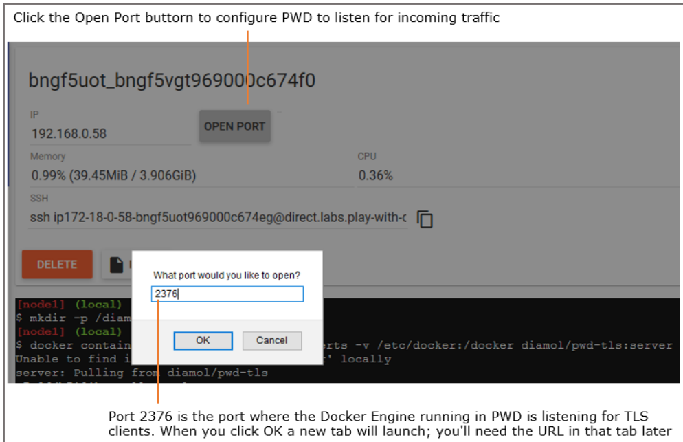
Figure 15.6 Opening ports in PWD lets you send external traffic into containers and the Docker Engine
