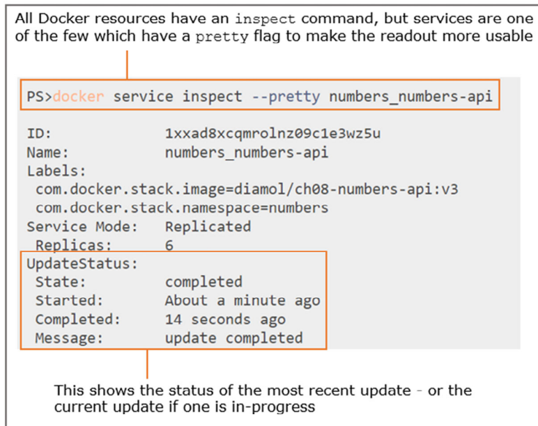
Figure 14.5 Inspecting a service shows the current configuration and the most recent update status
