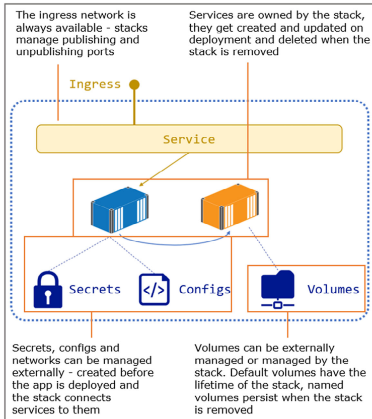
Figure 13.13 How Docker Swarm resources are managed by stack deployments
