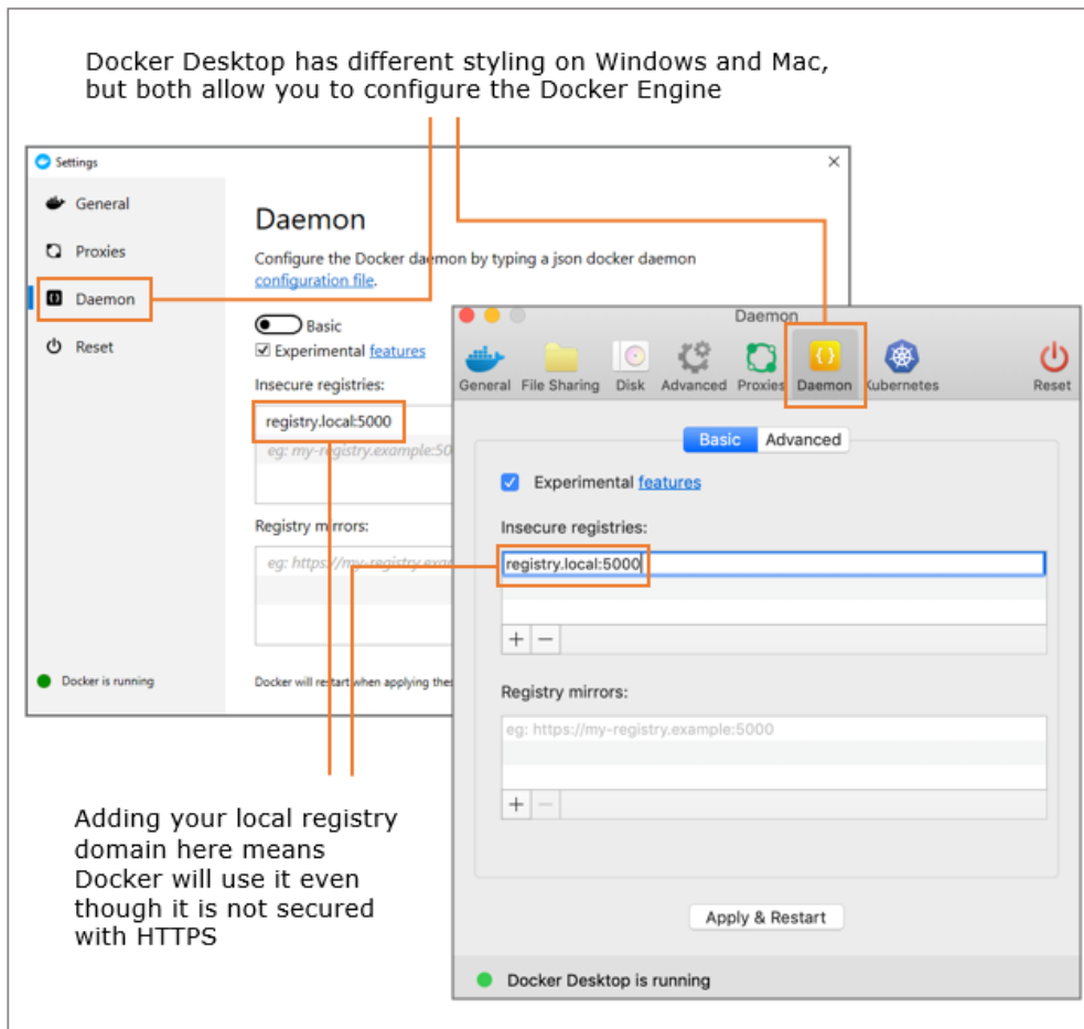
Figure 5.5 Allowing an insecure registry to be used in Docker Desktop
