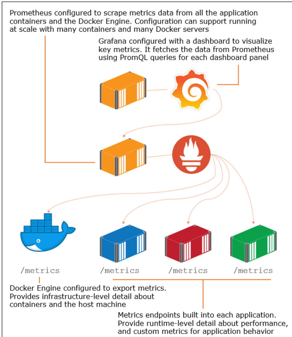
Figure 9.17 The architecture of monitoring in a containerized application - Prometheus is at the center
