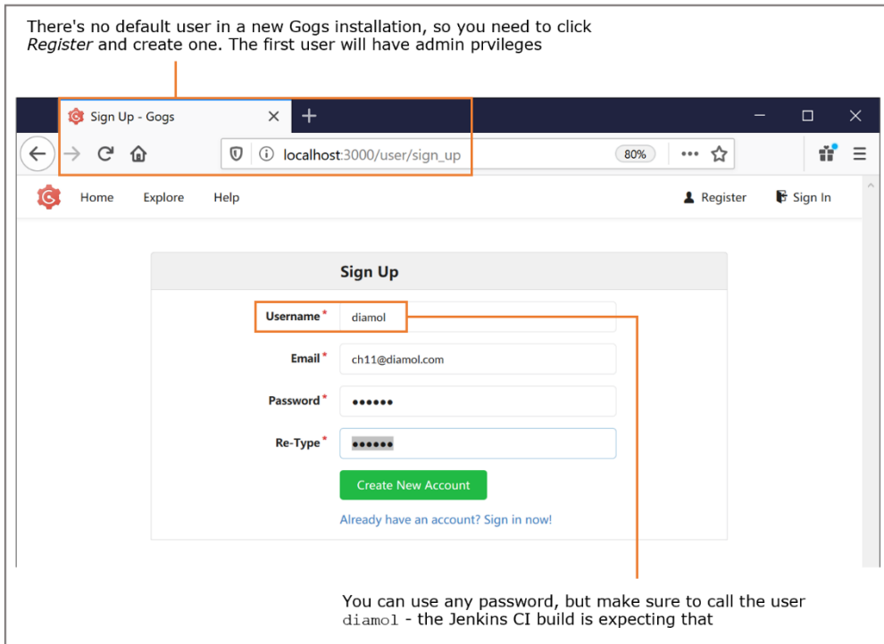
Figure 11.4 Creating a new user in Gogs which you can use to push source code to the server
