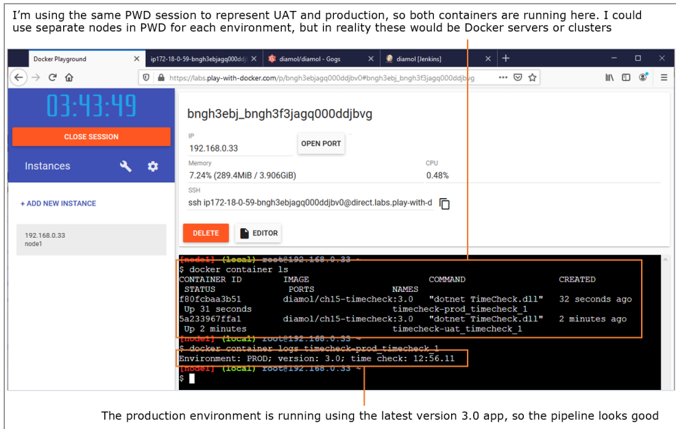
Figure 15.15 The deployment on PWD - to use a real cluster I'd just change the domain name and certs
