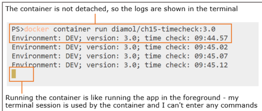
Figure 19.1 A container in the foreground takes over the terminal session until it exits
