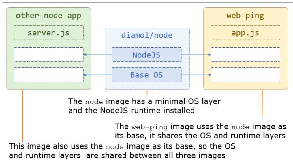
Figure 3.8 How image layers are logically built into Docker images
