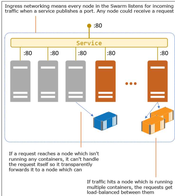
Figure 12.15 Docker Swarm uses ingress networking to route traffic to containers on nodes
