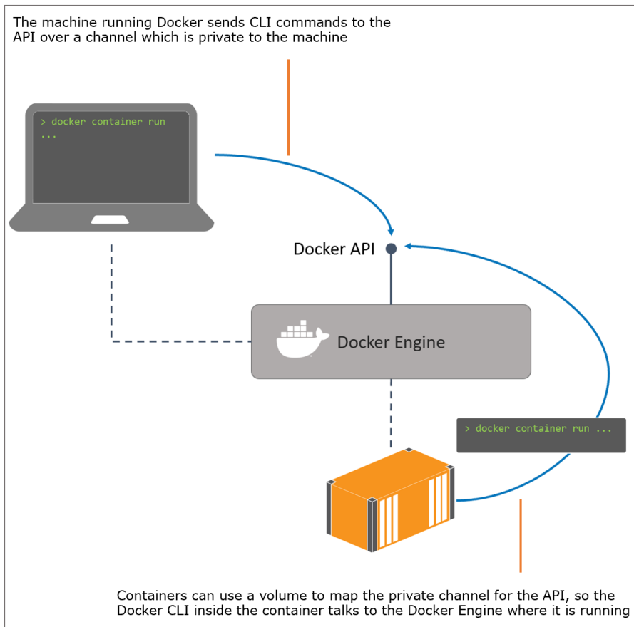
Figure 11.9 Running containers with a volume to bind the private channel for the Docker API
