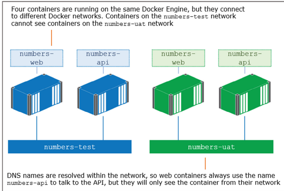
Figure 10.7 Running multiple environments on one Docker Engine, using networks for isolation
