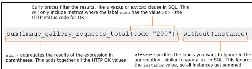
Figure 9.11 A simple Prometheus query. You don't need to learn much more PromQL than this.
