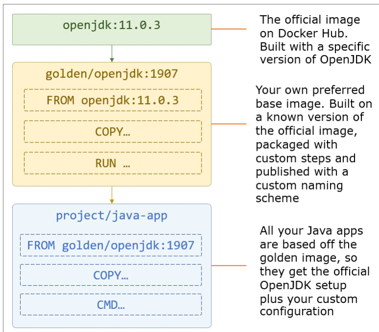
Figure 5.8 Using a golden image to encapsulate an official image
