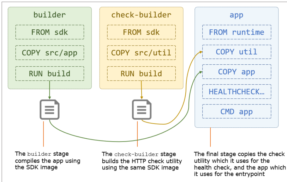
Figure 8.6 Using multi-stage builds to compile and package utilities alongside the application
