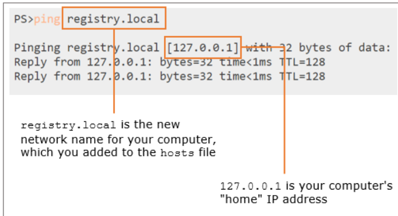
Figure 5.4 Adding a new network alias for your computer
