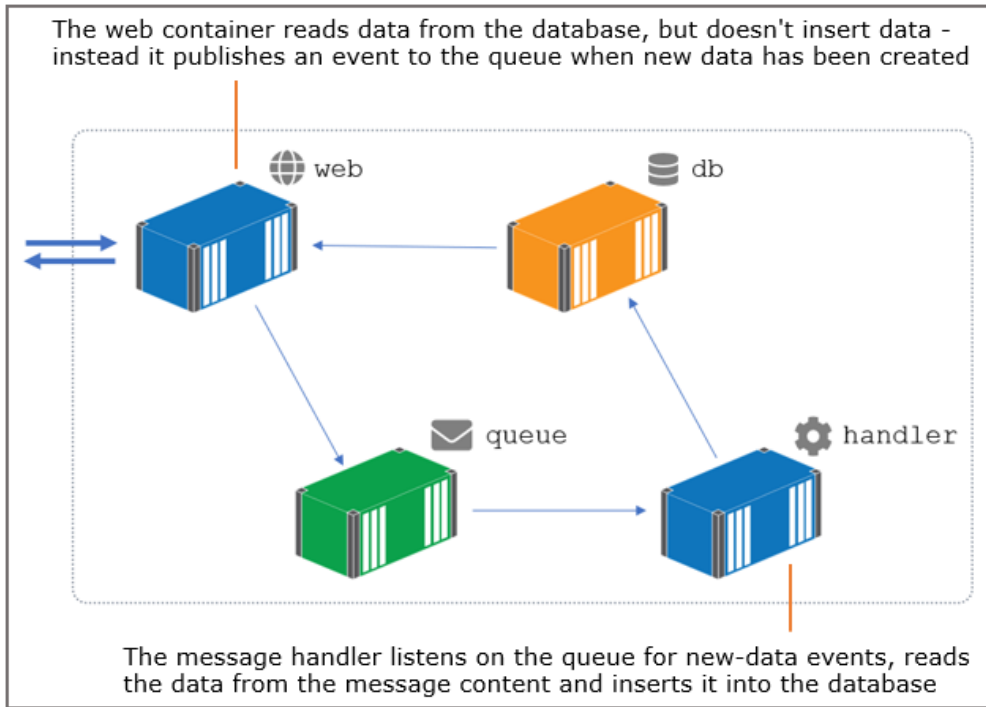
Figure 21.8 Asynchronous processing uses a message handler as well as an event publisher
