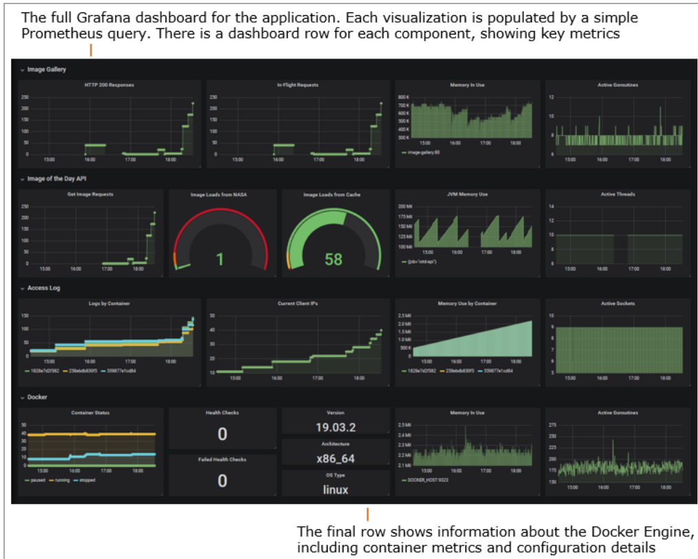
Figure 9.12 The Grafana dashboard for the application. Looks fancy but is actually pretty simple to build.
