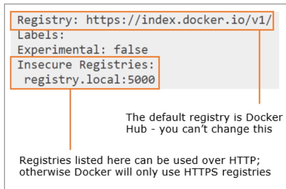
Figure 5.6 Insecure registries allowed for Docker to use
