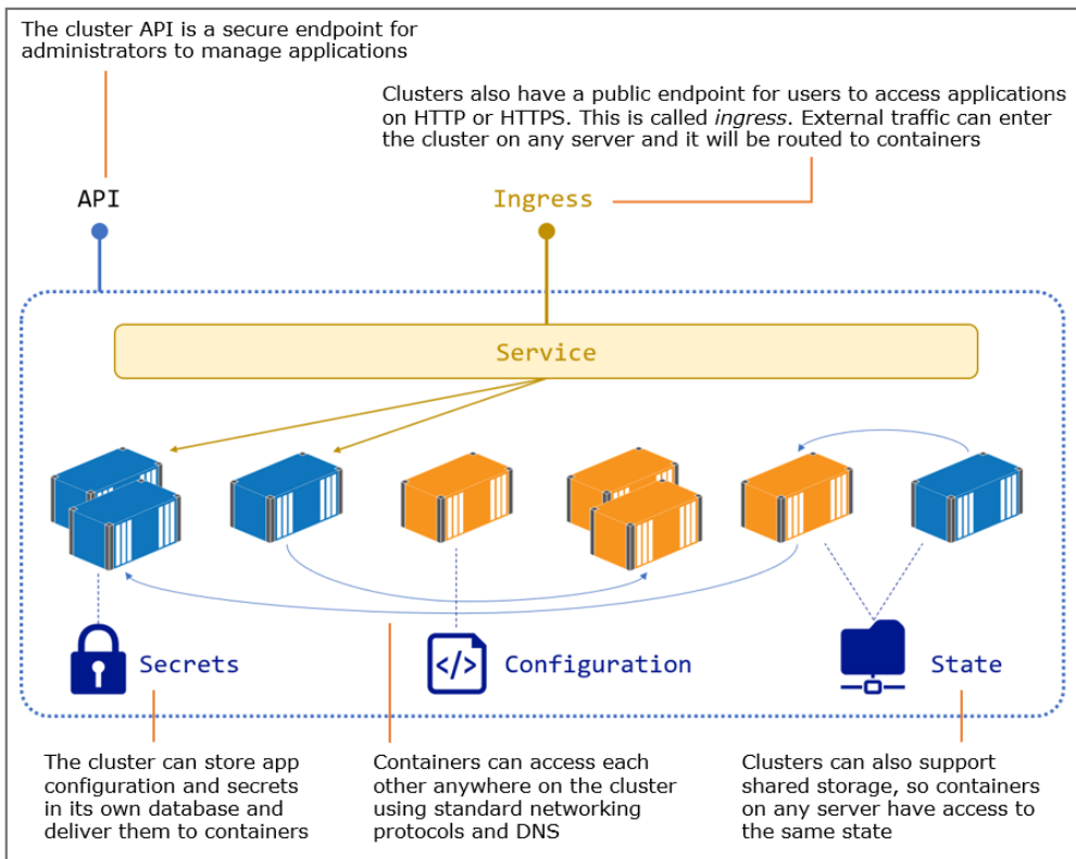
Figure 12.2 Orchestrators provide extra features for containers - networking, configuration and storage
