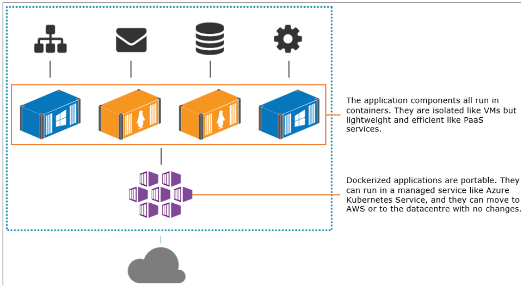
Figure 1.2 The same app migrated to Docker before moving to the cloud. This application has the cost benefits of PaaS with the portability benefits of IaaS and the ease of use you only get with Docker
