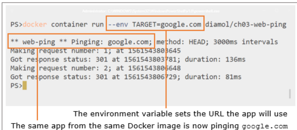
Figure 3.3. A container from the same image, sending traffic to Google
