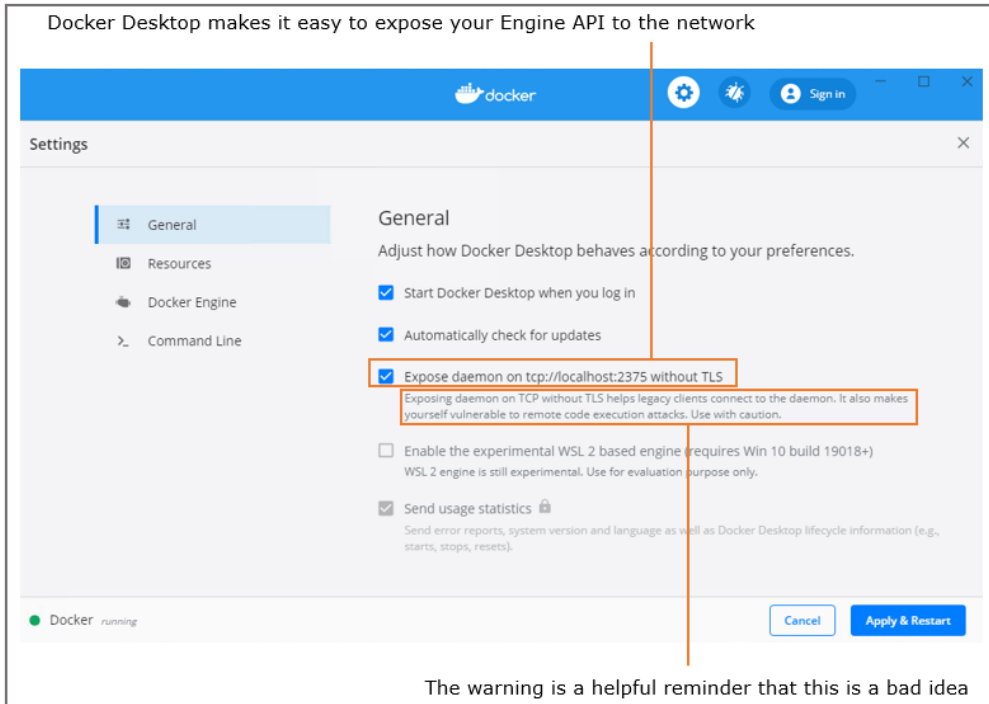
Figure 15.1 Enabling plain HTTP access to the Docker API - you should try and forget you saw this
