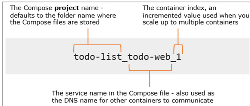
Figure 10.2 Docker Compose builds names for the resources it manages which include the project name
