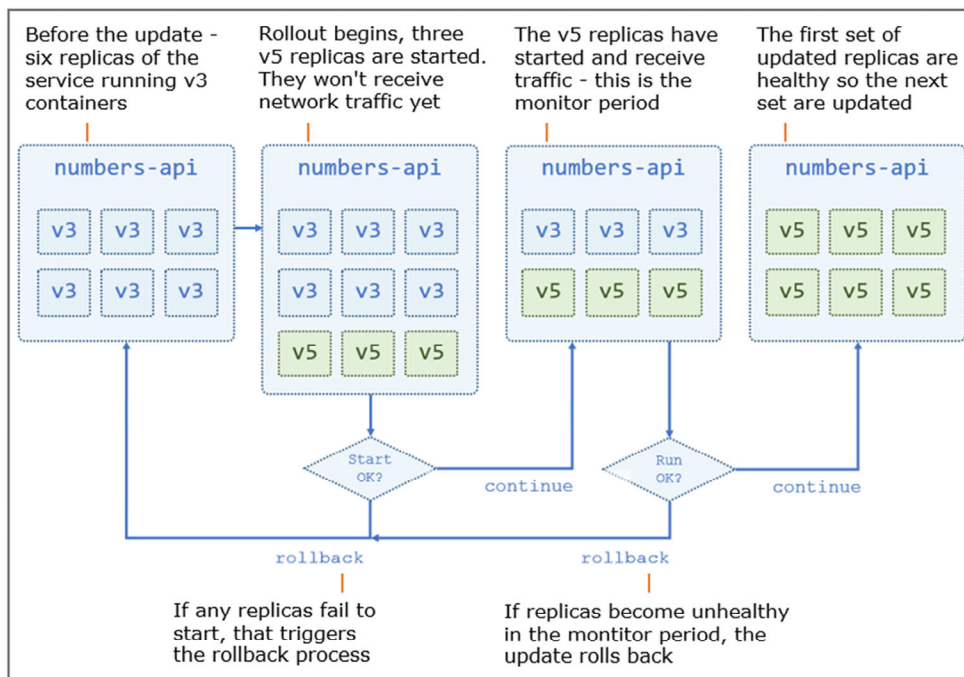
Figure 14.9 Looks suspiciously like a flowchart, but it's just a useful way to model the update process
