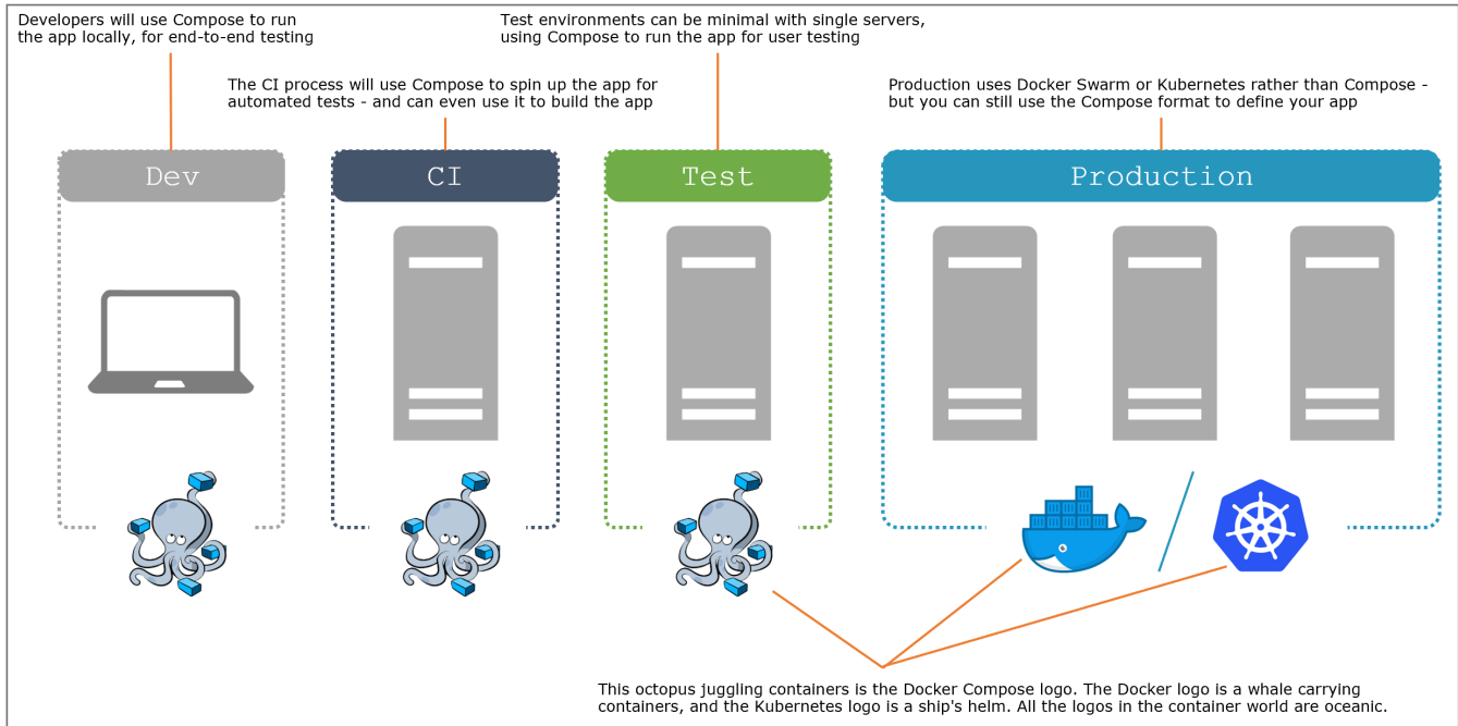
Figure 7.12 Where you use Docker Compose in the application lifecycle from dev to production
