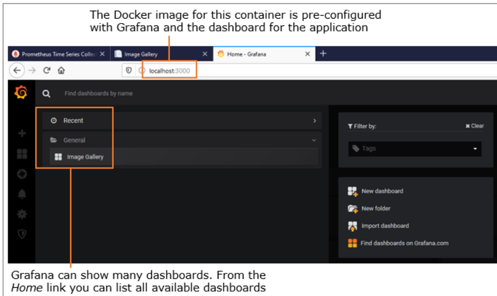
Figure 9.13 Navigating dashboards in Grafana - all the available dash
