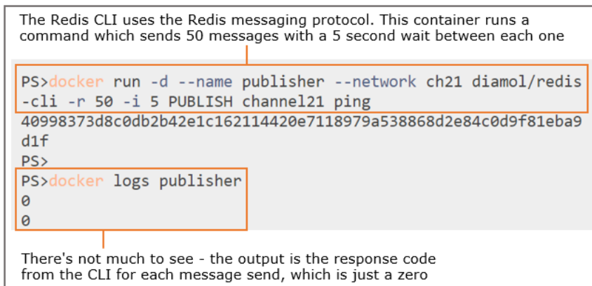
Figure 21.3 The Redis CLI is a simple way to send messages to the queue running in the Redis container
