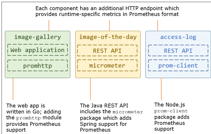
Figure 9.5 Prometheus client libraries in your apps make the metrics endpoint available in the container
