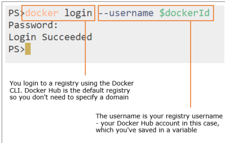
Figure 5.2 Logging in to Docker Hub
