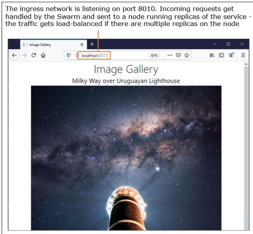
Figure 12.17 Published ports in services use the ingress network and Swarm routes requests to replicas
