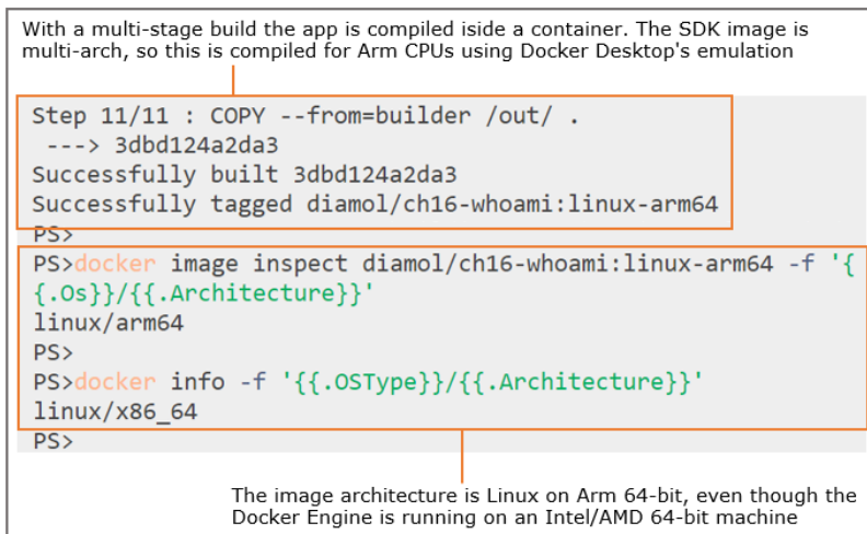
Figure 16.2 Cross-platform support, building Arm images from Intel machines using emulation
