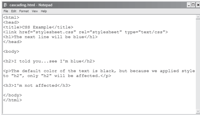
Figure 7-1: Calling an external style sheet that affects the <h1> , <h2> , and <h3> tags
