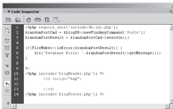
Figure 14-2: Adding the command execution and error handling
