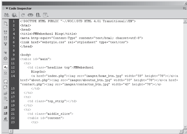
Figure 12-2: Source code of blogHeader.php
