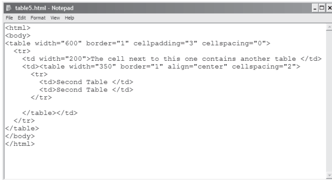
Figure 6-53: Table inside a table
