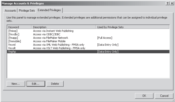
Figure 5-48: The fmphp privilege set defined
