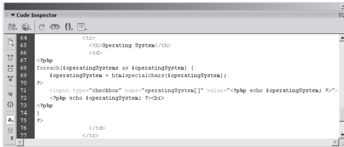
Figure 17-22: Source code for the Operating System check box set
