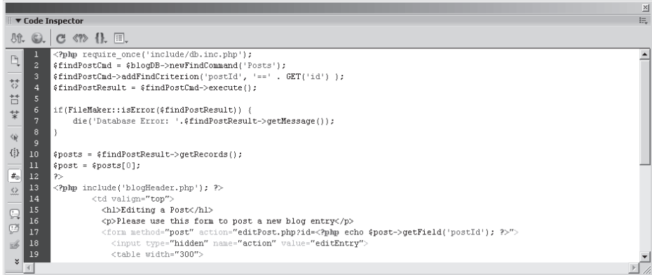
Figure 15-6: FileMaker API find for a single post
