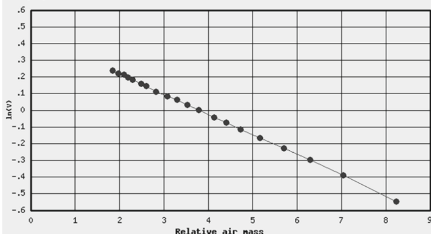
Langley Plot for sun photometer calibration
