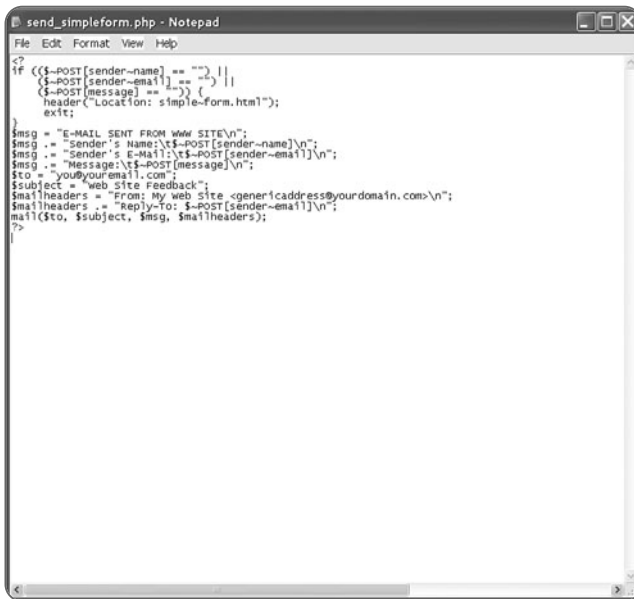
Figure 8.2 The mail script.
