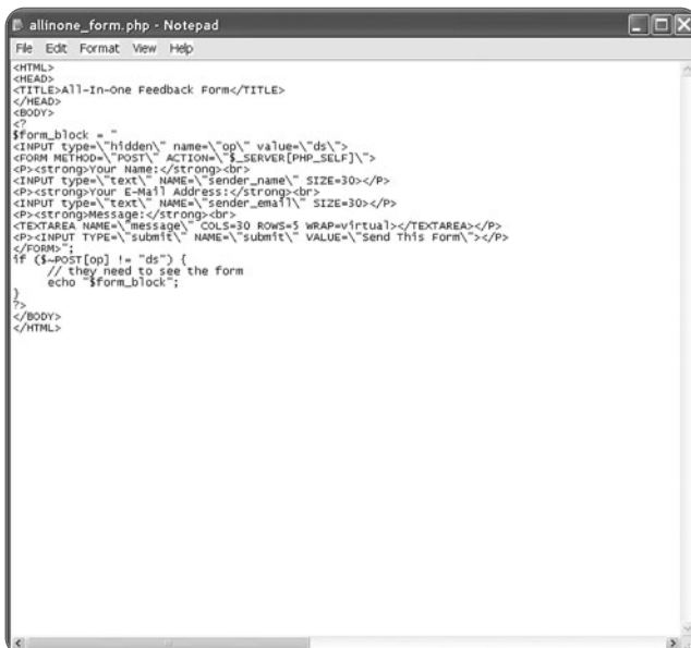
Figure 8.7 The all-in-one script.
