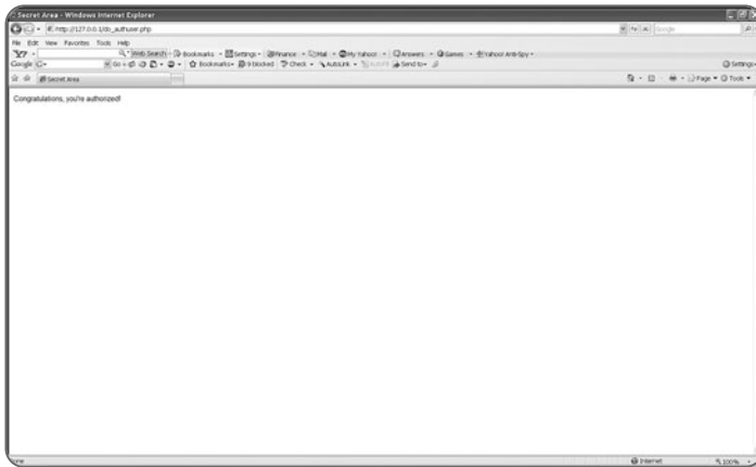
Figure 15.8 Successful login!
