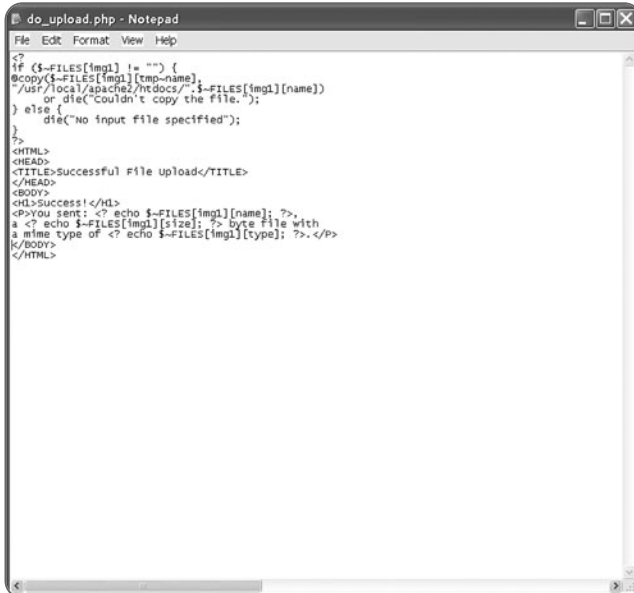
Figure 10.2 The upload script.
