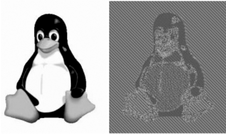
Figure 15–2. Wikipedia's illustration of the pattern flow in ECB mode encryption. This image is licensed under the GNU Free Documentation License at http://www.gnu.org/copyleft/fdl.html . It is from the Wikipedia article “Block Cipher Modes of Operation” at http://en.wikipedia.org/wiki/Block_cipher_modes_of_operation .
