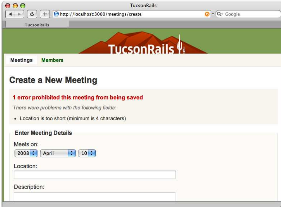
Figure 6.1: Validation errors
