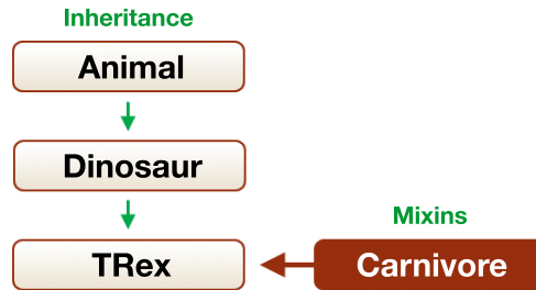
Figure 3.1: Method organization
