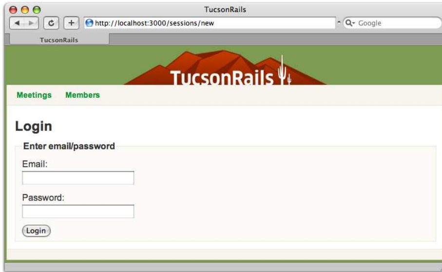
Figure 7.6: Login form
