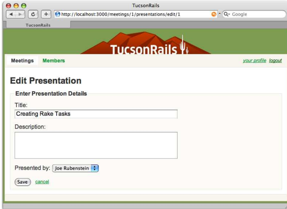
Figure 8.2: Editing presentations
