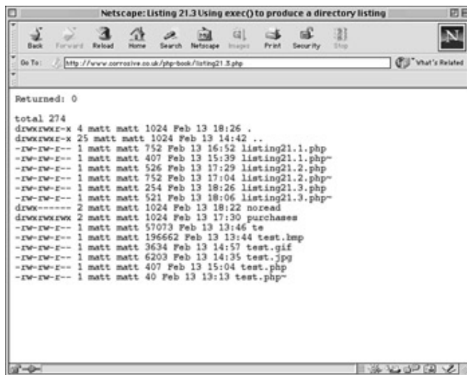
Figure 21.2: Using exec() to produce a directory listing.
