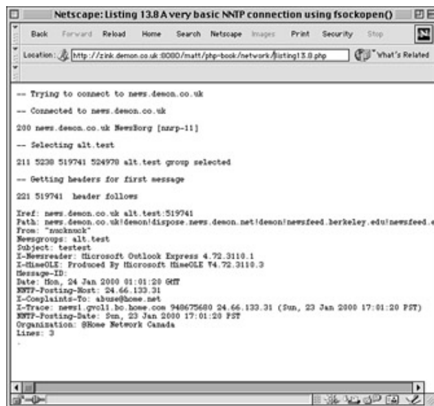
Figure 13.3: Making an NNTP connection.
