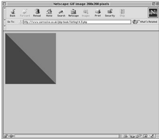
Figure 14.3: Using imagefill() .
