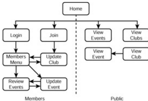
Figure 23.1: Application structure.
