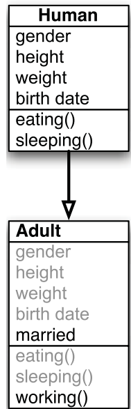
Figure 7.5 The Adult class can have all the same members as Human , while adding its own.
