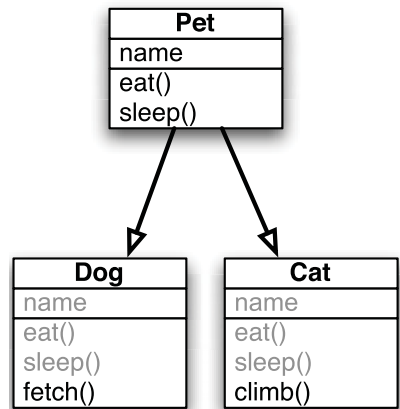
Figure 7.6 How the pet-cat-dog relationship would be implemented objectively.
