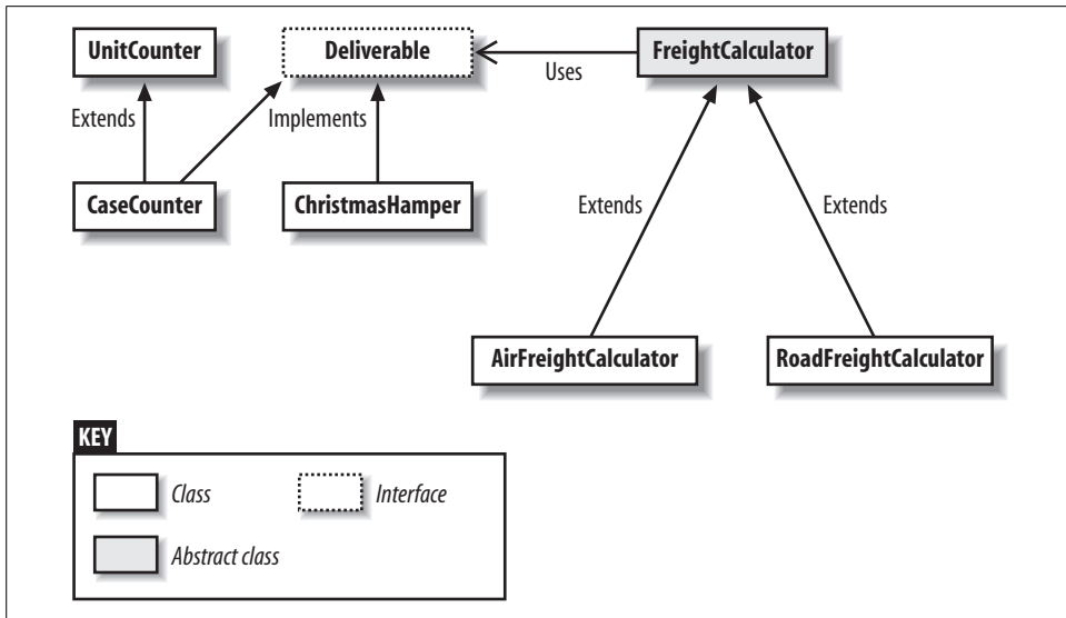
Figure 14-3. Class diagram
