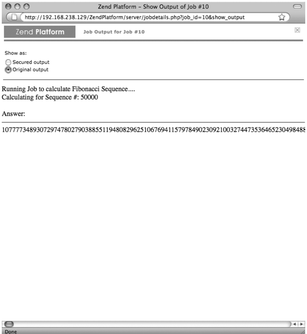
Figure 5-9. The output of the fibonacci.php script from the Job Queue console
