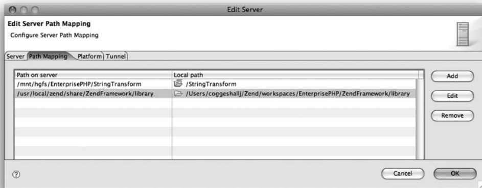
Figure 2-11. Server path mapping for the StringTransform project
