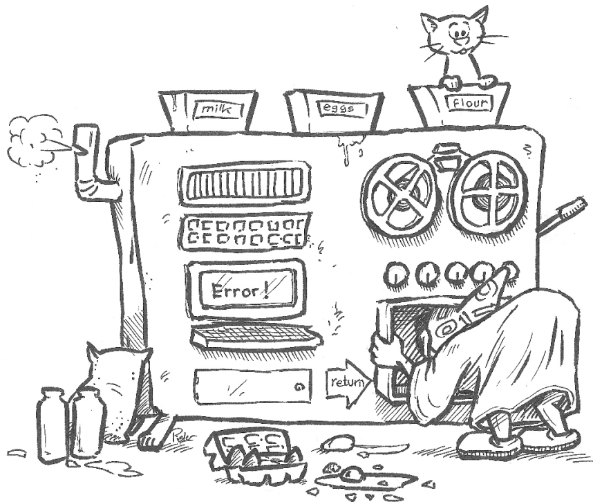
listing0807.py
